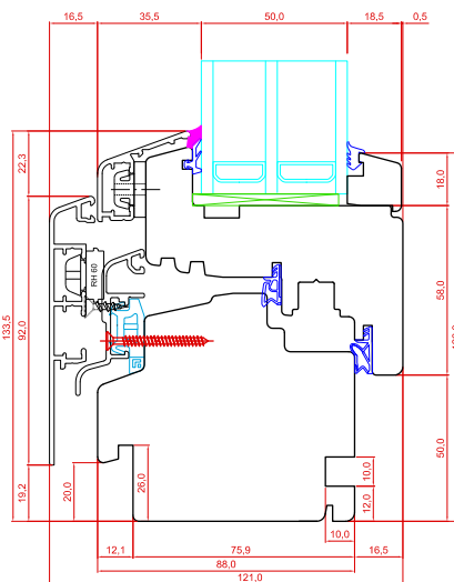
Vertical cross-section of the Viking Passive Style Window
